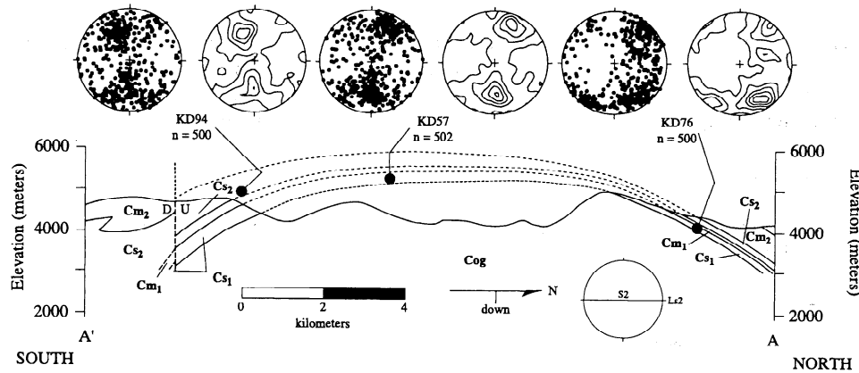
Figure 5. Quartz c -axis fabrics of samples discussed in text projected into the central part of the N-S cross section (see Plate 2). Lower hemisphere, equal area projections, geographic orientation of stereonets, orientation of S2 and Ls2, and number of c -axes measured are indicated. Contour intervals are 1, 2, 3, 4, and 5 times uniform distribution. See Table 1 and Figure 4 for location of samples.
