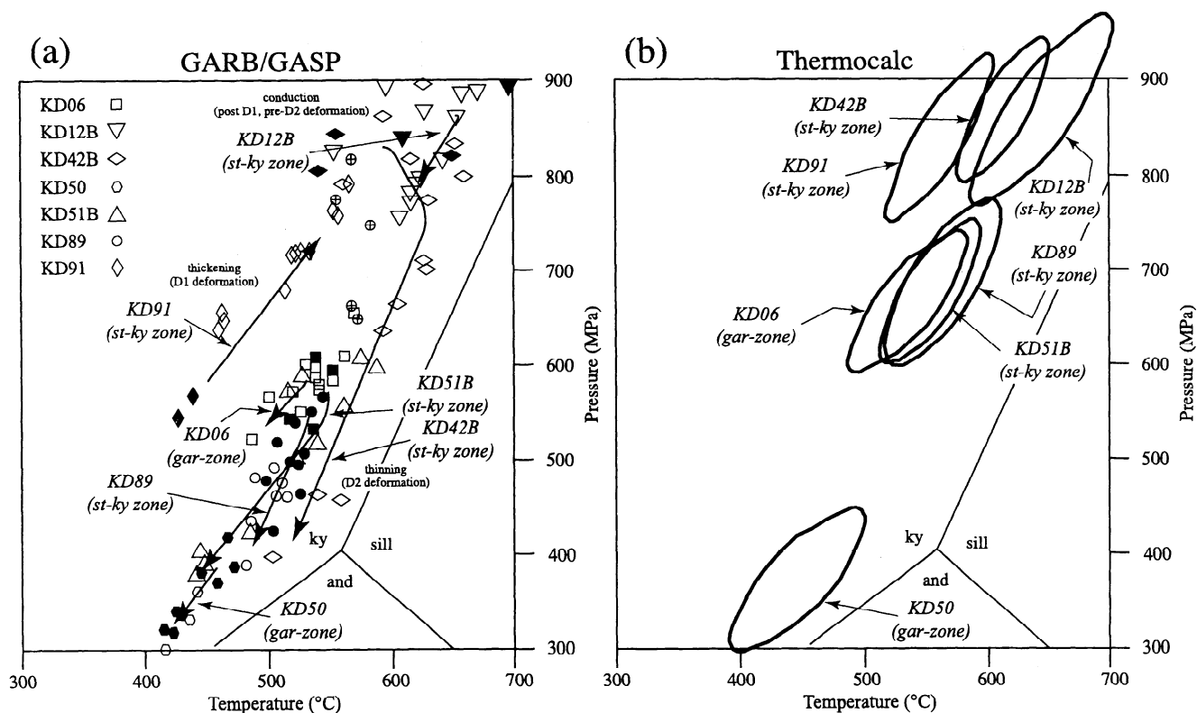
Figure 7. PT diagrams showing the results of thermobarometry analyses of pelites. (a) Garnet-biotite (GARB) temperatures and garnet-kyanite-quartz-plagioclase (GASP) pressures. Mineral rims are given by open symbols; mineral cores are given by solid symbols with crosses; mineral inclusions are given by solid symbols. PT paths inferred from variation in rim pressures and temperatures are illustrated as solid lines. (b) Peak temperatures and pressures calculated from Thermocalc. Ellipses represent weighted mean temperatures and pressures for rim compositions for each sample. Here and, andalusite; gar, garnet; ky, kyanite; sill, sillimanite; st, staurolite. Aluminosilicate stability fields are from Bohlen et al. [1991]. Peak PT conditions calculated from Thermocalc are projected on a N-S cross section in Figure 8; sample locations are shown in Table 1 and Figure 4.
