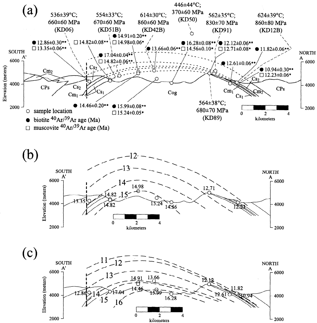
Figure 8. (a) Thermobarometric, based on Thermocalc, and mica ^{40}\text{Ar}/^{39}\text{Ar} geochronology results projected onto the central part of the N-S cross section (see Plate 1). Thermobarometric sample numbers are in parenthesis. Ages are given in Ma and errors are 1 sigma; weighted mean plateau ages are indicated by asterisks; preferred ages are indicated by double asterisks. See Figures 10 and 11 for age spectra. (b) Isochrons of muscovite ^{40}\text{Ar}/^{39}\text{Ar} plateau and preferred ages projected on the central part of the N-S cross section. (c) Isochrons of biotite ^{40}\text{Ar}/^{39}\text{Ar} preferred ages projected on the central part of the N-S cross section.
