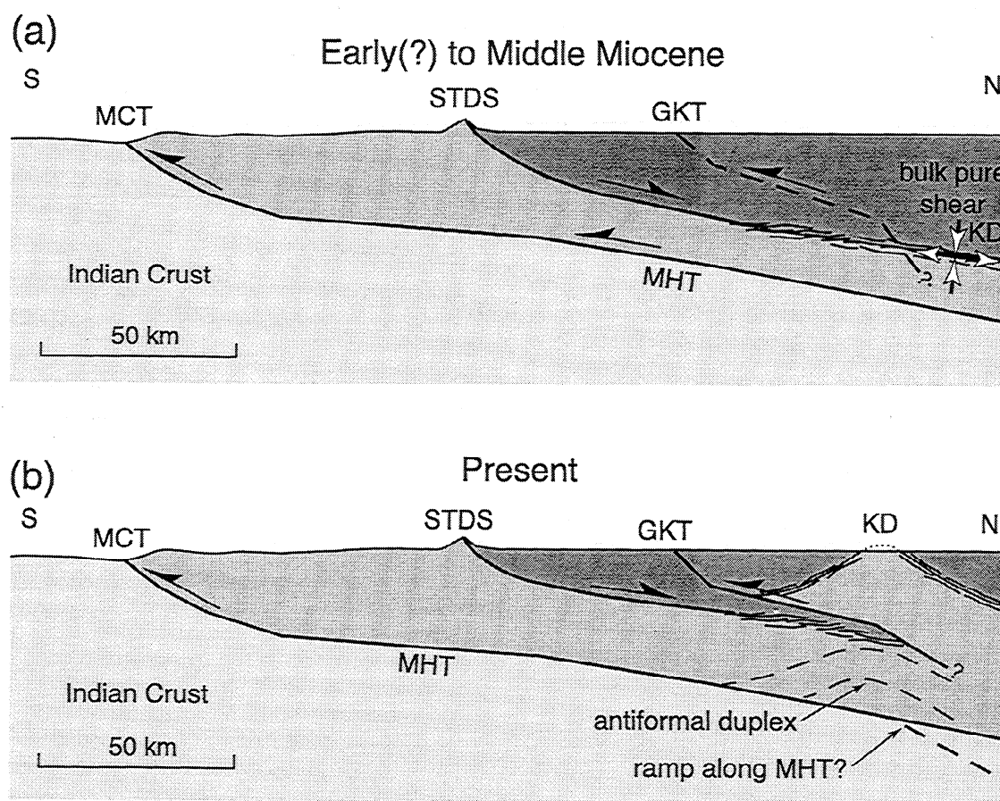
Figure 13. Interpretative, schematic, evolutionary N-S cross sections across the Himalaya and southern Tibet at the longitude of the Kangmar Dome. (a) Configuration of major structures and D2 extensional fabrics in the Kangmar Dome during the early(?) to middle Miocene. (b) Configuration of major structures at present. See text for details. Modified from Hauck et al. [1998], Wu et al. [1998], and Makovsky et al. [1999]. GKT, Gyirong-Kangmar thrust fault system; KD, Kangmar Dome; MCT, Main Central Thrust; MHT, Main Himalayan Thrust; STDS, Southern Tibetan Detachment System.
