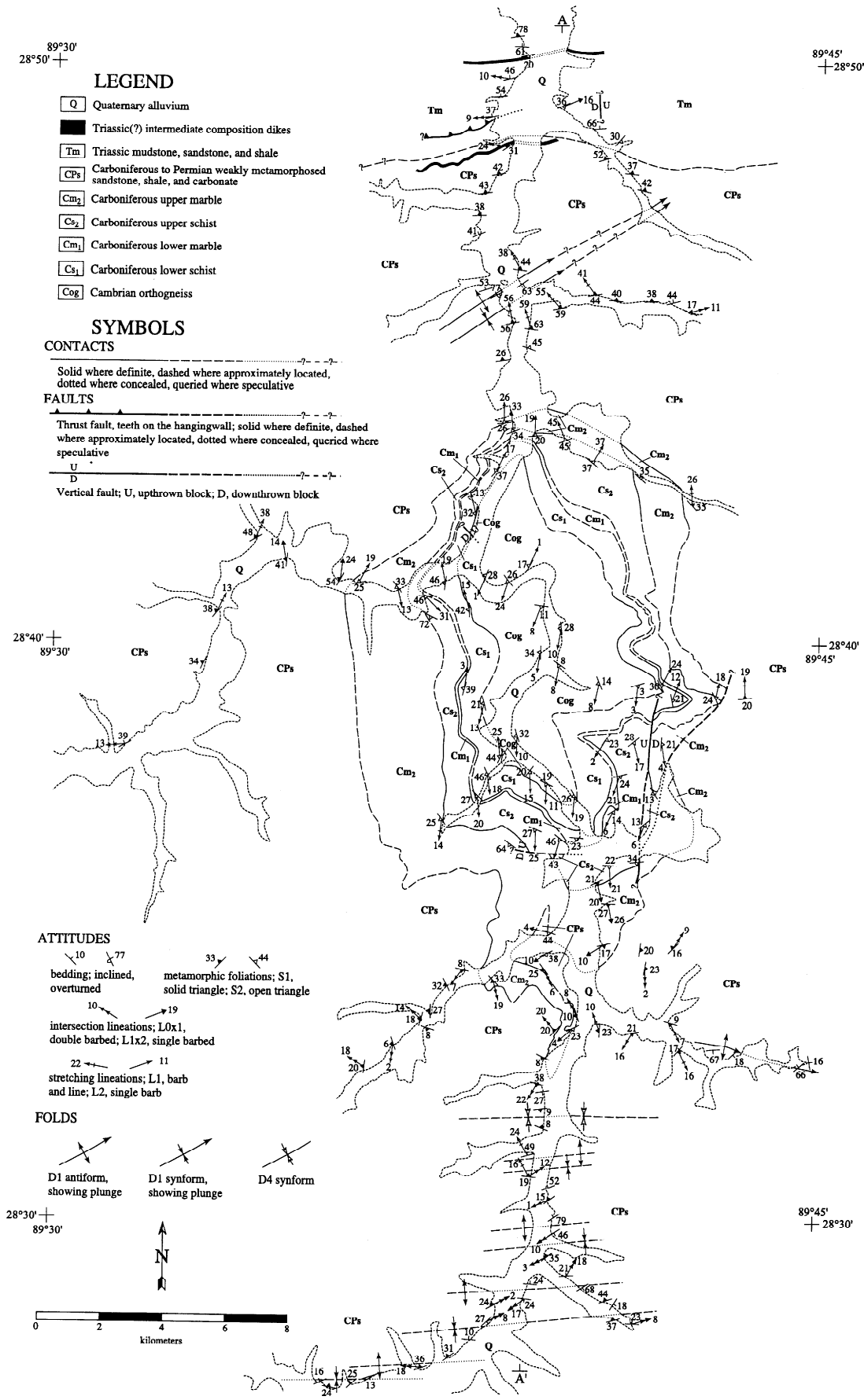
Plate 1. Simplified geologic map of the Kangmar Dome.
