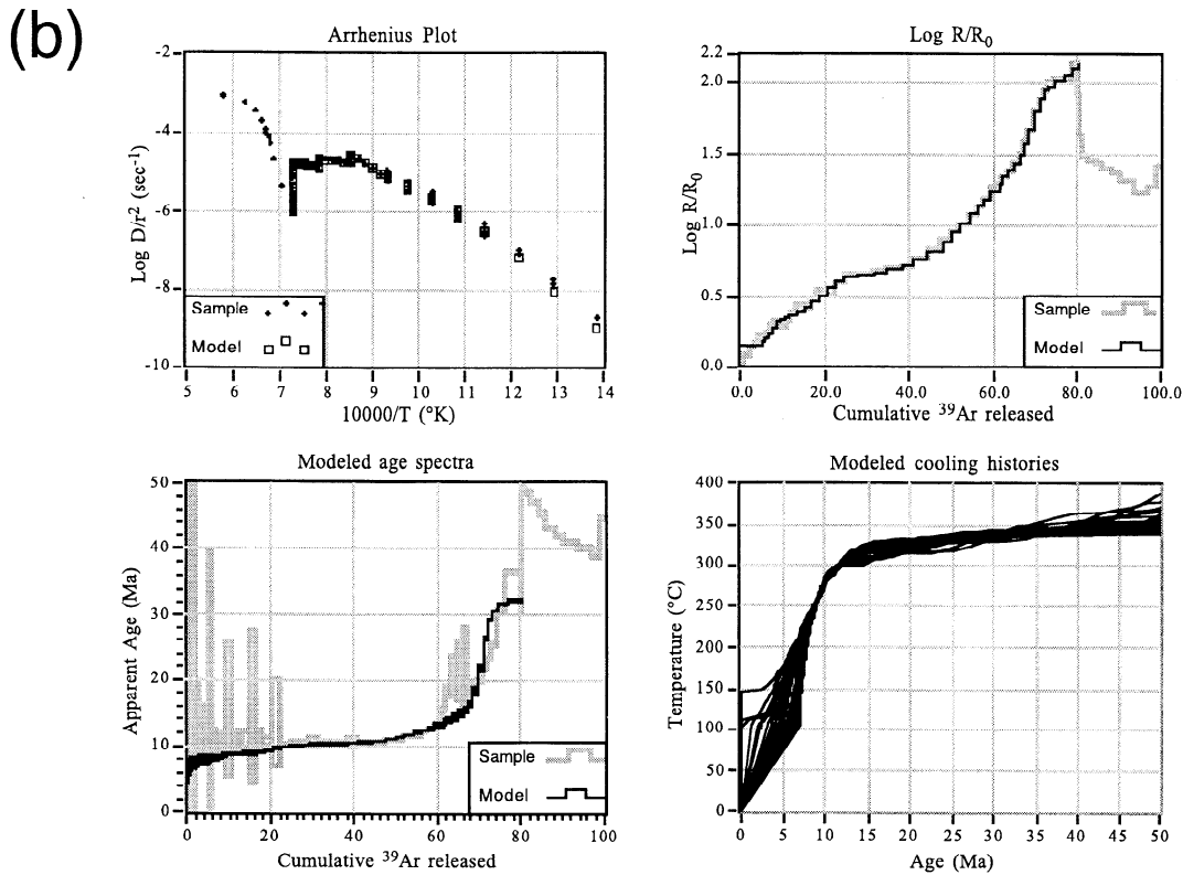
Figure 12. (a) Potassium feldspar ^{40}\text{Ar}/^{39}\text{Ar} age spectra and apatitic fission track ages (open diamonds) projected onto the central part of the N-S cross section (see Plate 2). (b) Example of diffusion domain modeling showing Arrhenius plot, \text{log } R/R_0 plot, release spectra, and range of cooling histories for sample KD20.
