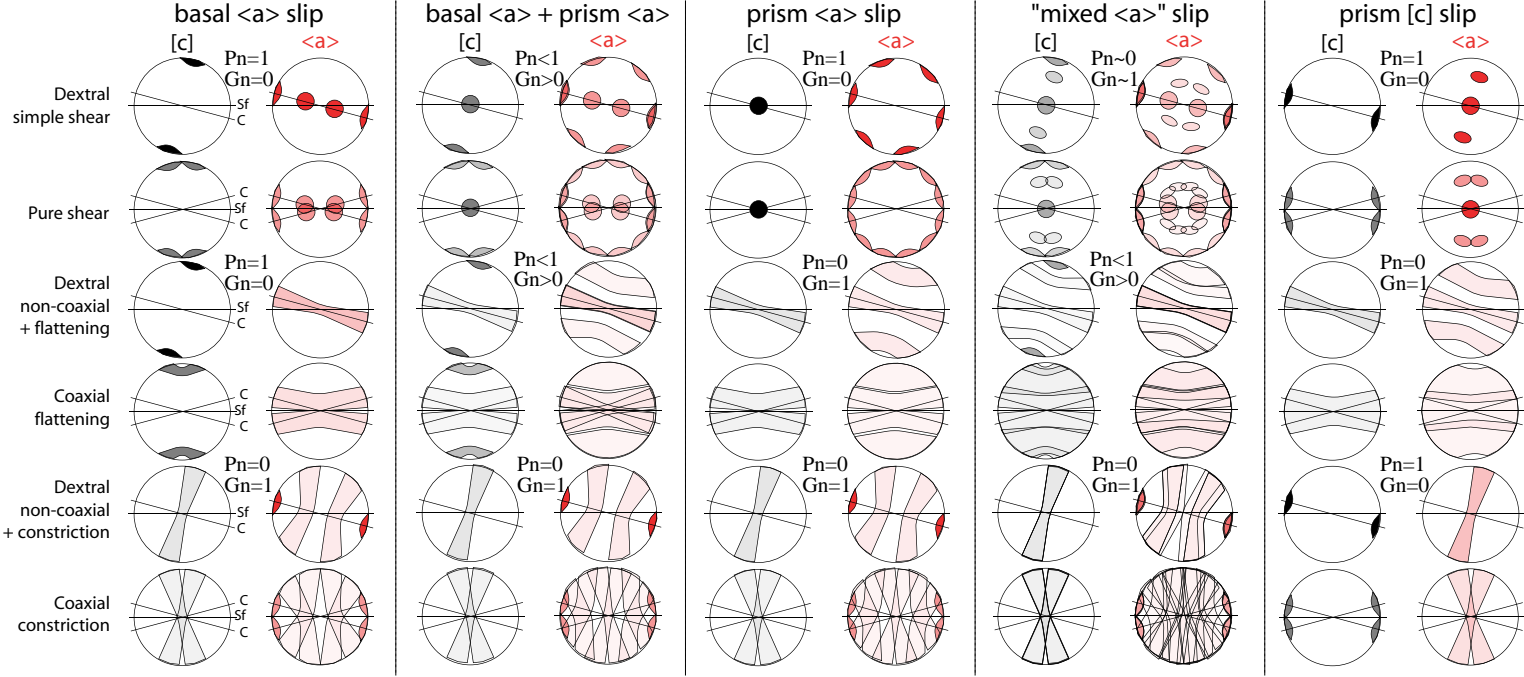
Fig. 1. CPOs and normalized point ( P_n ) and girdle ( G_n ) indices expected from various quartz slip systems subjected to different strain geometries. In each stereonet, foliation (Sf) is horizontal, shear/cisaillement (C) planes are inclined, and lineation is at the intersection of the foliation with the primitive (i.e. east-west).
