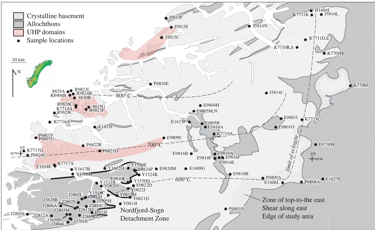
Fig. 2. The Western Gneiss region of Norway consists of a crystalline basement overlain by allochthons emplaced toward the SE. Major features include the ultrahigh-pressure (UHP) domains, the top-to-the-west Nordfjord–Sogn Detachment Zone and the top-to-the-east shear zone along the eastern edge of the crystalline basement. Peak metamorphic temperatures increase toward the NW (Kylander-Clark et al. 2008); the CPOs reported here reflect either these or lower temperatures.
