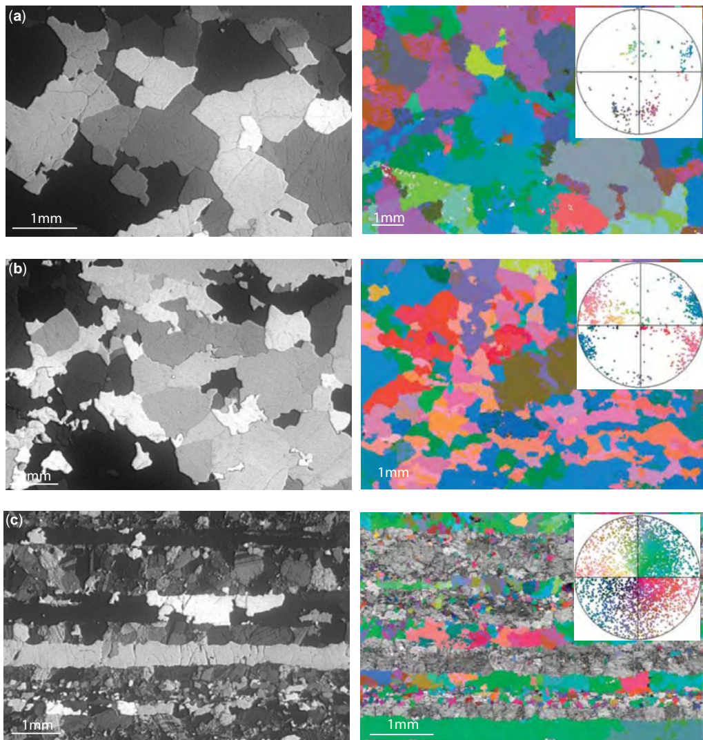
Fig. 3. Representative microstructures. Optical microstructures (left) are indicative of quartz deformation regime 2 (a few samples) or 3 (most samples); cross-polarized light. EBSD map coloured by one-point-per-grain quartz crystal orientations shown in inset c -axis stereonet. (a) Quartz vein P6807F7 showing weak undulatory extinction, weak sub-grain formation, and fairly straight grain boundaries indicative of quartz deformation regime 3. (b) Quartz vein in eclogite K7717A2 showing weak undulatory extinction, modest sub-grain formation, and straight grain boundaries indicative of regime 3. (c) Gneiss sample R9823F9 composed of bands of quartz and plagioclase.
