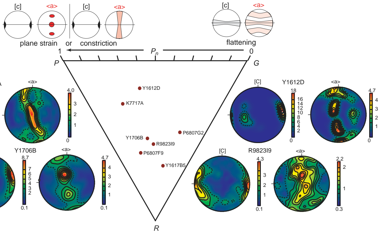
Fig. 4. (Continued) (d) CPOs attributable to prism [c] slip are compatible with either plane strain (e.g. Y1706B) or constriction (e.g. K7717A).
