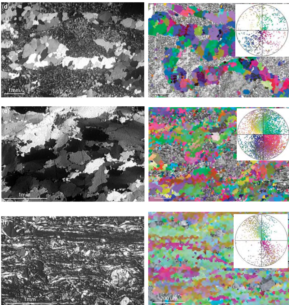
Fig. 3. (Continued). Regime 3. (d) Gneiss sample P6821D1 with quartz-rich zones surrounded by fine-grained symplectites. Grain boundaries are dentate. Regime 3. (e) Gneiss sample P6803A2 with strong undulatory extinction, strong sub-grain formation, and dentate grain boundaries indicative of sub-grain rotation recrystallization (regime 2). (f) Quartz-rich ultramylonite J3701E3 with highly stretched quartz grains and feldspar porphyroclasts. Regime 2.
