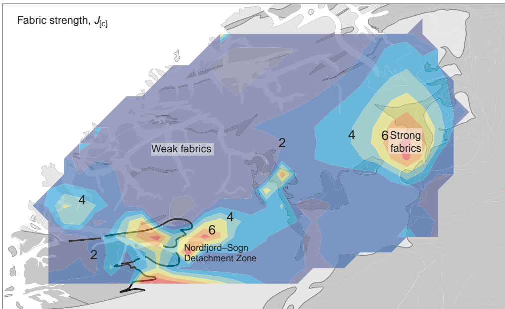
Fig. 6. As measured by J_{c|} value ( J_{(a)} is nearly identical and 1 - R is similar), CPOs are strongest along the Nordfjord–Sogn Detachment Zone and within the top-to-the-east domain in the east. Contoured using the Matlab griddata(cubic) routine.
