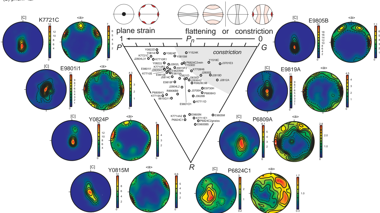
Fig. 4. (Continued) (b) CPOs attributable to prism <a> glide have characteristics compatible with a mix of plane strain and constriction, with the former dominant; none are compatible with flattening.
