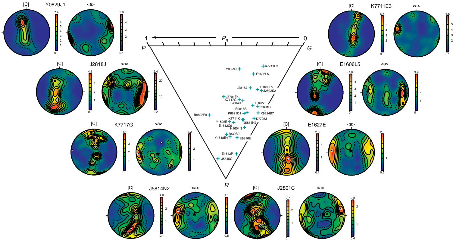
Fig. 4. (Continued) (c) CPOs attributable to ‘mixed \langle a \rangle ’ slip are compatible with constriction and plane strain.
