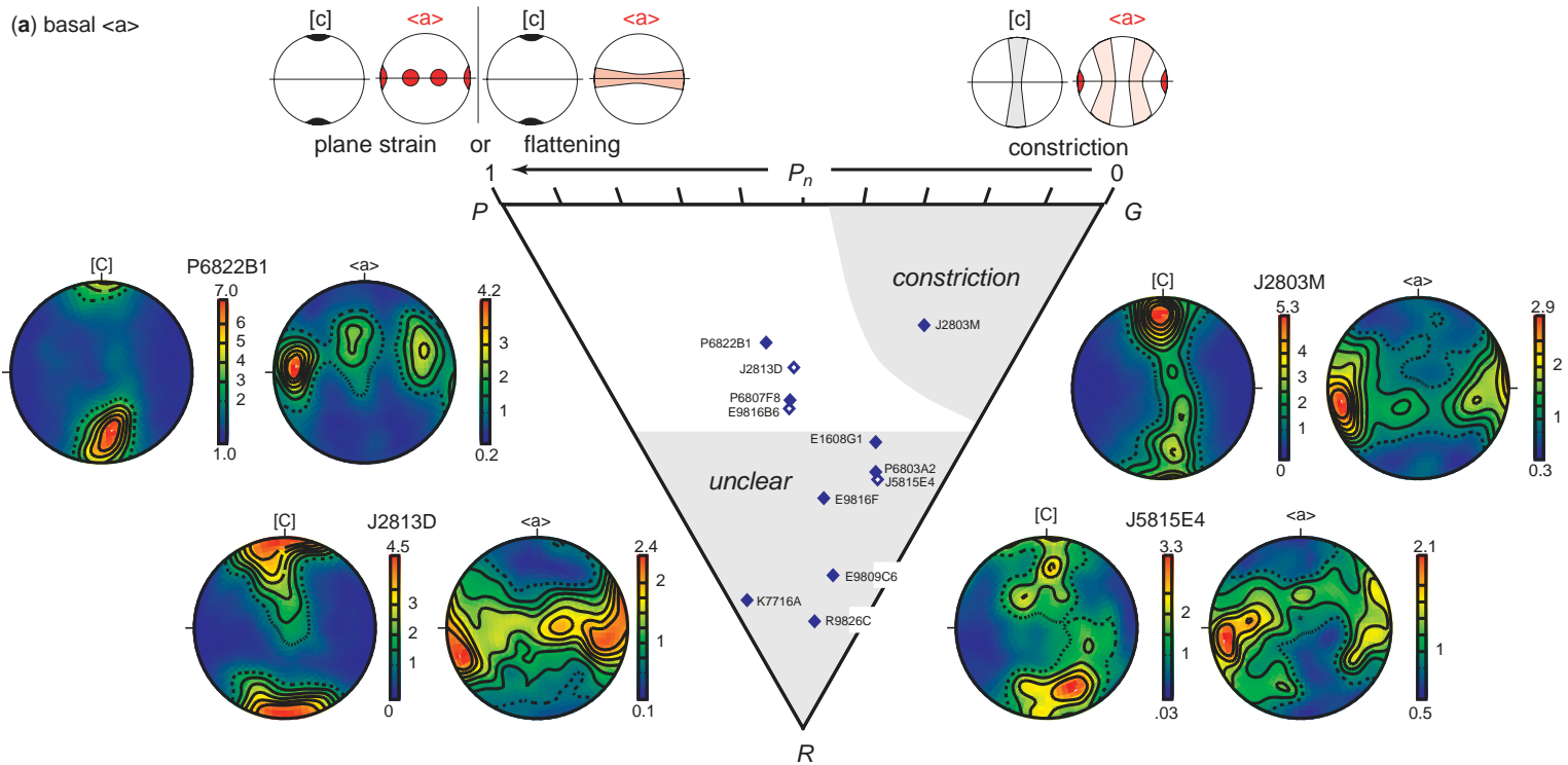
Fig. 4. Representative quartz CPOs and calculated P , G and R values. Upper hemisphere projections in which the \langle a \rangle axes have been collapsed using 622 symmetry. CPOs for other 'J' and 'Y' samples can be found in Johnston et al. (2007b) and Young (2005), respectively. (a) CPOs attributable to basal \langle a \rangle glide have characteristics compatible with plane strain or flattening (4 samples) and constriction (1 sample); another seven samples have more obscure CPOs with high R values.
