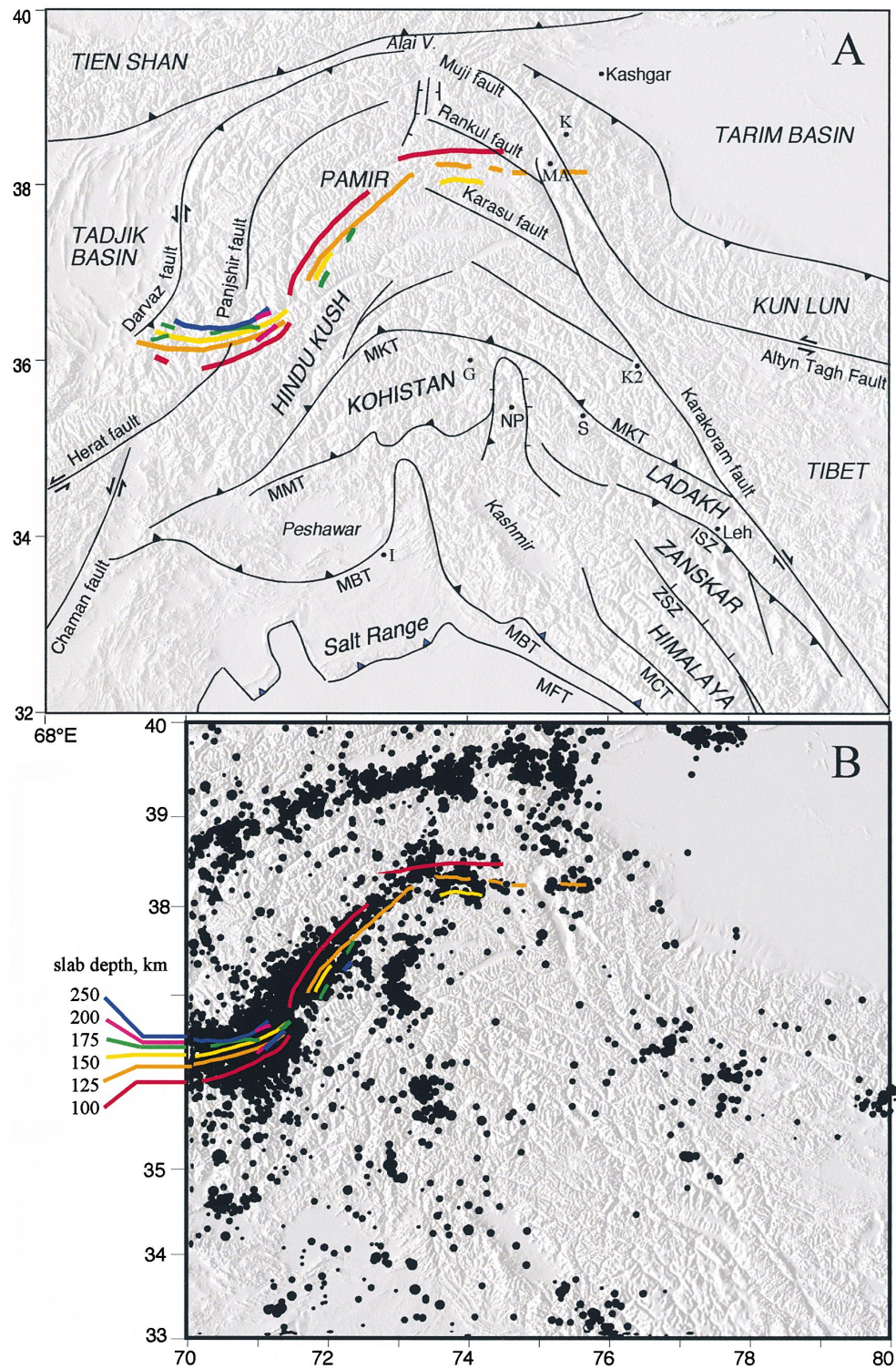
Figure 3. A, Digital topographic elevation map and a structural map of the western Himalaya, Hindu Kush, Pamir, Karakoram, and western Tibet, which also shows the major structures and the location of the Hindu Kush deep seismic zone. NP, Nanga Parbat; MKT, Main Karakoram thrust; ISZ, Indus suture zone; MMT, Main mantle thrust; ZSZ, Zaskar shear zone; MCT, Main central thrust; MBT, Main boundary thrust; I, Islamabad; S, Skardu; K and MA are the Kongur and Muztagh Ata gneiss domes between the dextral Karakoram Fault and the sinistral Altyn Tagh Fault at the far western end of Tibet. B, Map of the Hindu Kush, Pamir, Karakoram, and western Himalaya showing all seismicity covering the period 1964–1992 and depth contours, from 100 to 250 km, of the Hindu Kush seismic zone (after Pegler and Das 1998).
