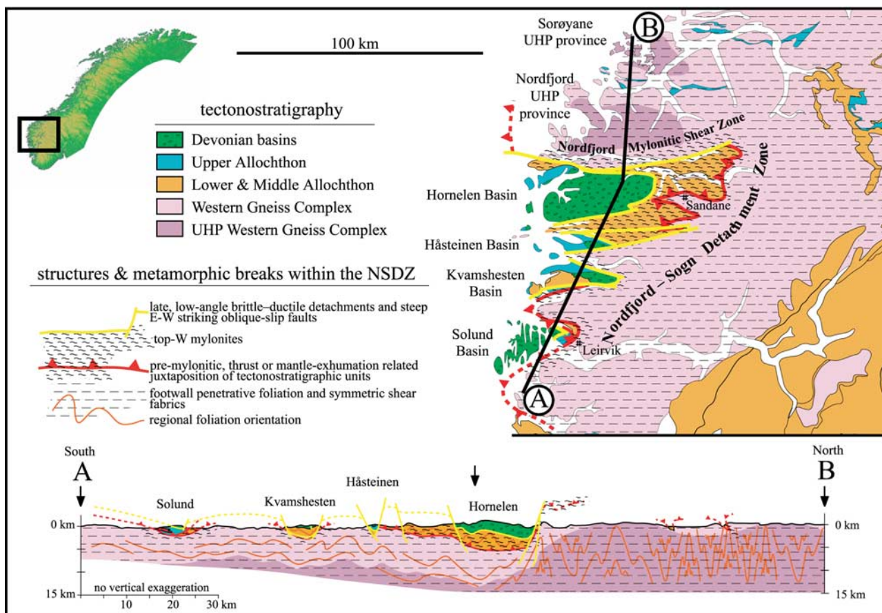
Figure 1. Regional map and extension-perpendicular cross section displaying tectonostratigraphic relationships and structural styles associated with the Nordfjord-Sogn Detachment Zone.
