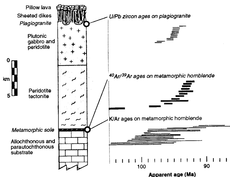
Fig. 1. Comparison of U/Pb zircon ages from plagiogranites (17) and ^{40}\text{Ar}/^{39}\text{Ar} ages (discussed here) and K/Ar ages (2, 9, 21, 22) from metamorphic sole hornblendes. The line for each age shows 2\sigma (U/Pb ages) or 1\sigma (K/Ar and ^{40}\text{Ar}/^{39}\text{Ar} ages) standard deviation of age uncertainty. Other units of the ophiolite substrate are shown in plain text.
