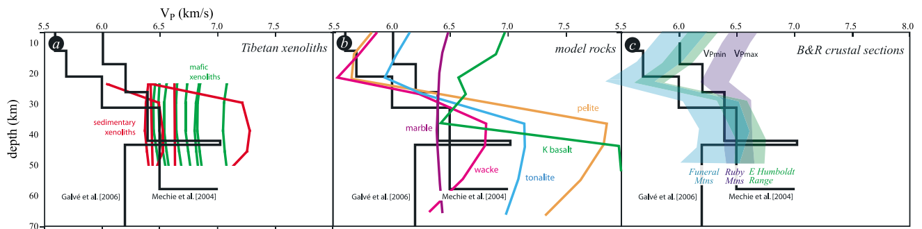
Figure 8. Observed V_P compared to V_P calculated for (a) Tibetan xenoliths, (b) model rocks, and (c) crustal sections. The correspondence is good for some metametamorphic xenoliths, for model quartzofeldspathic rocks at \leq 30 km, for marble at \geq 30 km, and for the Basin and Range crustal sections at all depths. Width of colored bar in Figure 8c shows range in V_P for different directions of wave propagation.
