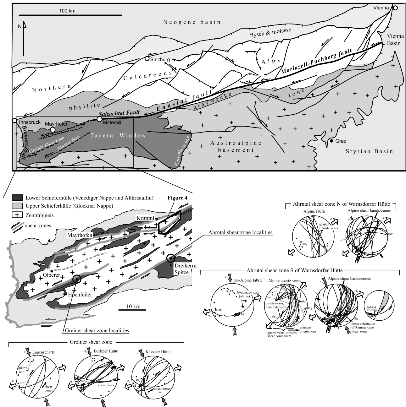
Figure 2. (a) The Salzachtal-Ennstal-Mariazell-Puchberg (SEMP) fault zone [after Linzer et al. , 2002] in the framework of the Tertiary tectonic structures of the central and eastern Eastern Alps and the location and structural and kinematic characterization of two (Greiner and Ahrntal) of the three major ductile shear zones of the interior of the central and western Tauern Window. The Rinderkarsee shear zone that connects to the SEMP is southeast of Krimml (geologic contacts after Bigi et al. [1990]). Structural data are plotted in lower hemisphere, equal-area stereograms, s_1 , first foliation; str_1 , first stretching lineations; e_3 to e_1 , principal strain directions.
