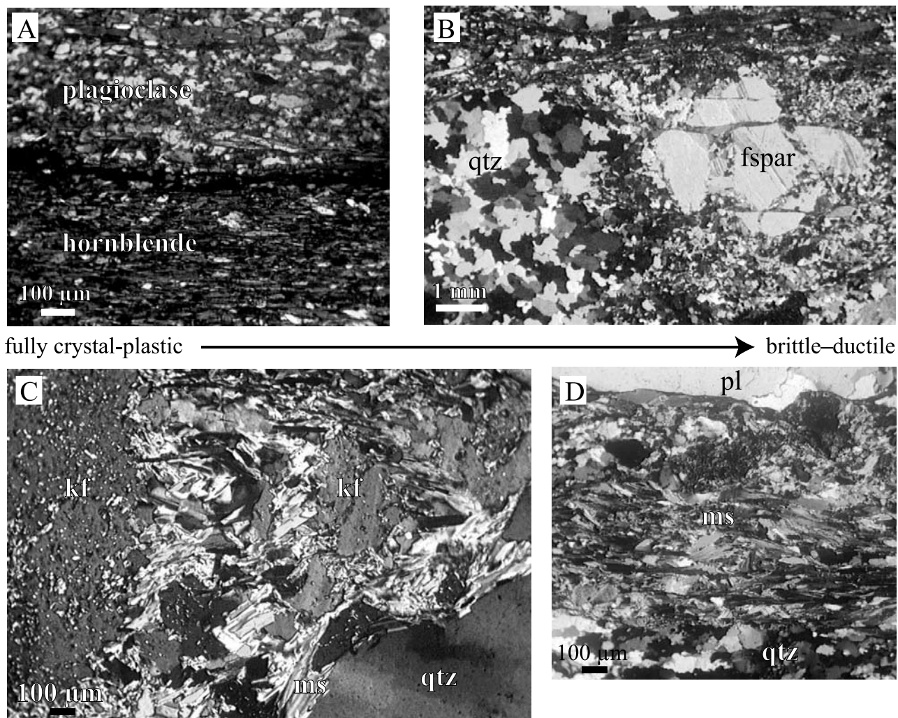
Figure 5. Rinderkarssee shear zone microstructures. (a) Mylonitic amphibolite from southern shear zone showing crystal-plastic deformation of amphibole and feldspar (sample 5729G1). (b) Brittle-ductile fabric in southern shear zone Zentralgneis with brittle feldspar and ductile quartz. Feldspar fractures are filled with recrystallized quartz, muscovite, and calcite (5729F1). (c) Alteration of K-feldspar to muscovite (5729H1B). (d) A more mature, millimeter-scale shear zone formed via the linkage of muscovite-rich grain boundaries. Cracking and fluid infiltration produced the reaction \text{K-feldspar} + \text{fluid} \rightarrow \text{muscovite} + \text{albite} . This muscovite-producing reaction served to drive both strain localization and dynamic recrystallization in K-feldspar via transformational plasticity.
